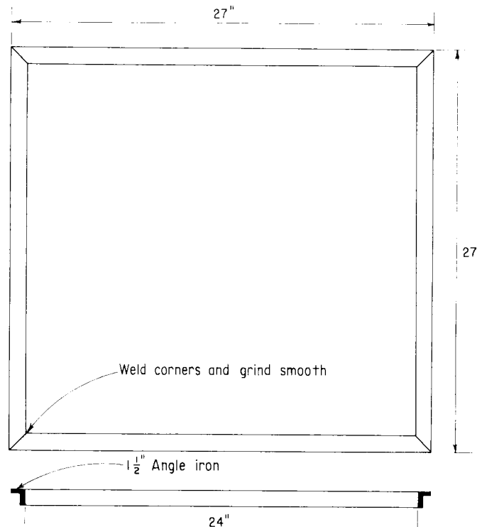
FIG. 1 Typical Metal Template for Excavating Test Pit
